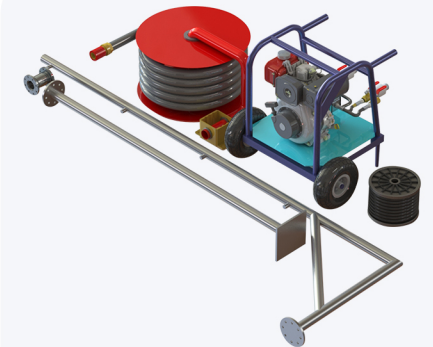
Oil Spill Dispersant Spray System
